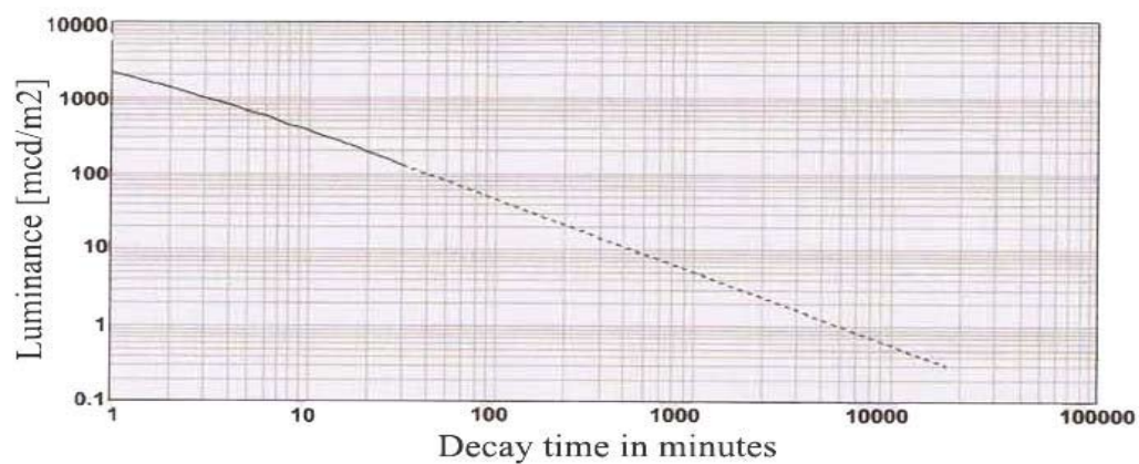
The CoreGLOW™ Stone afterglowing duration curve
